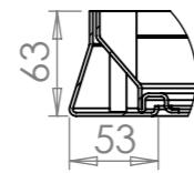
DETAIL B SCALE 1 : 5
