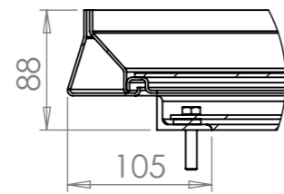
DETAIL B SCALE 1 : 5
